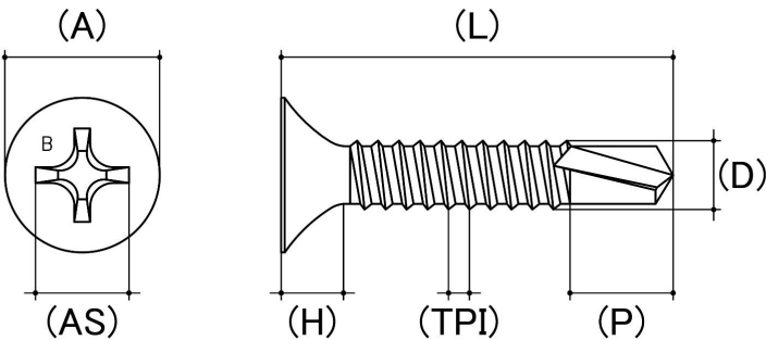
Cad Drawings shown for graphic representation only.*
